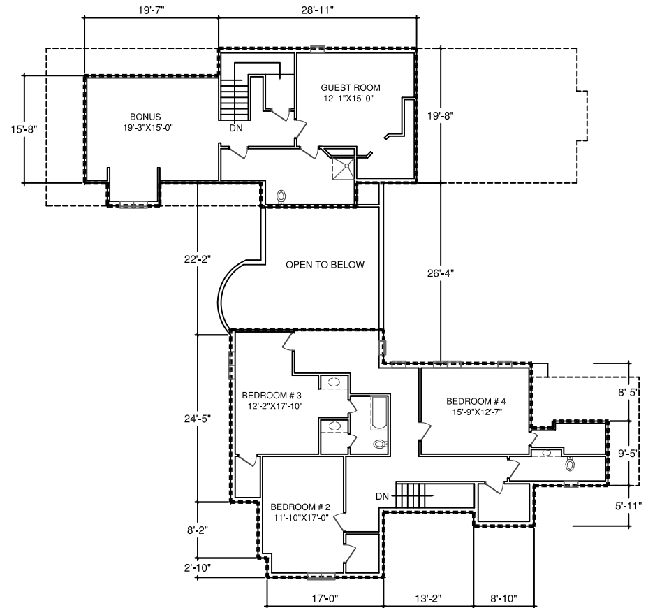
2nd floor 901 PATRICK JOHNSTON 1351/ 950 HEATED SQUARE FEET
