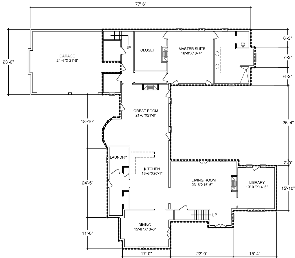
1st FLOOR 901 PATRICK JOHNSTON 2977 HEATED SQUARE FEET
